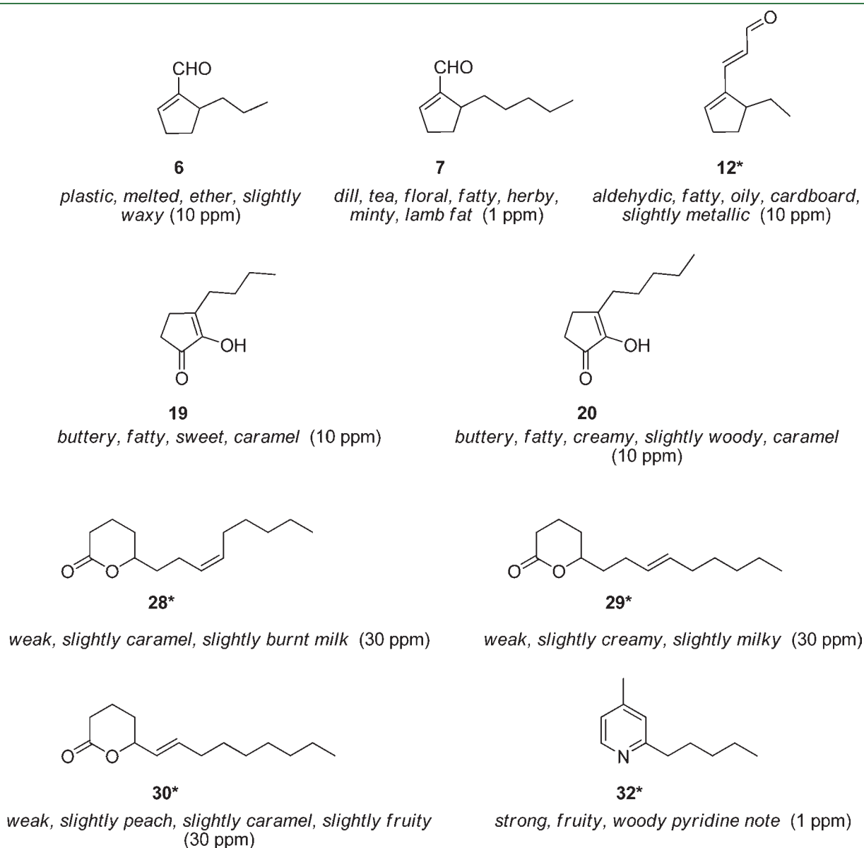
Figure 3. Molecules newly identified in chicken and their flavor description (in salted water 0.3%). *First natural occurrence.
