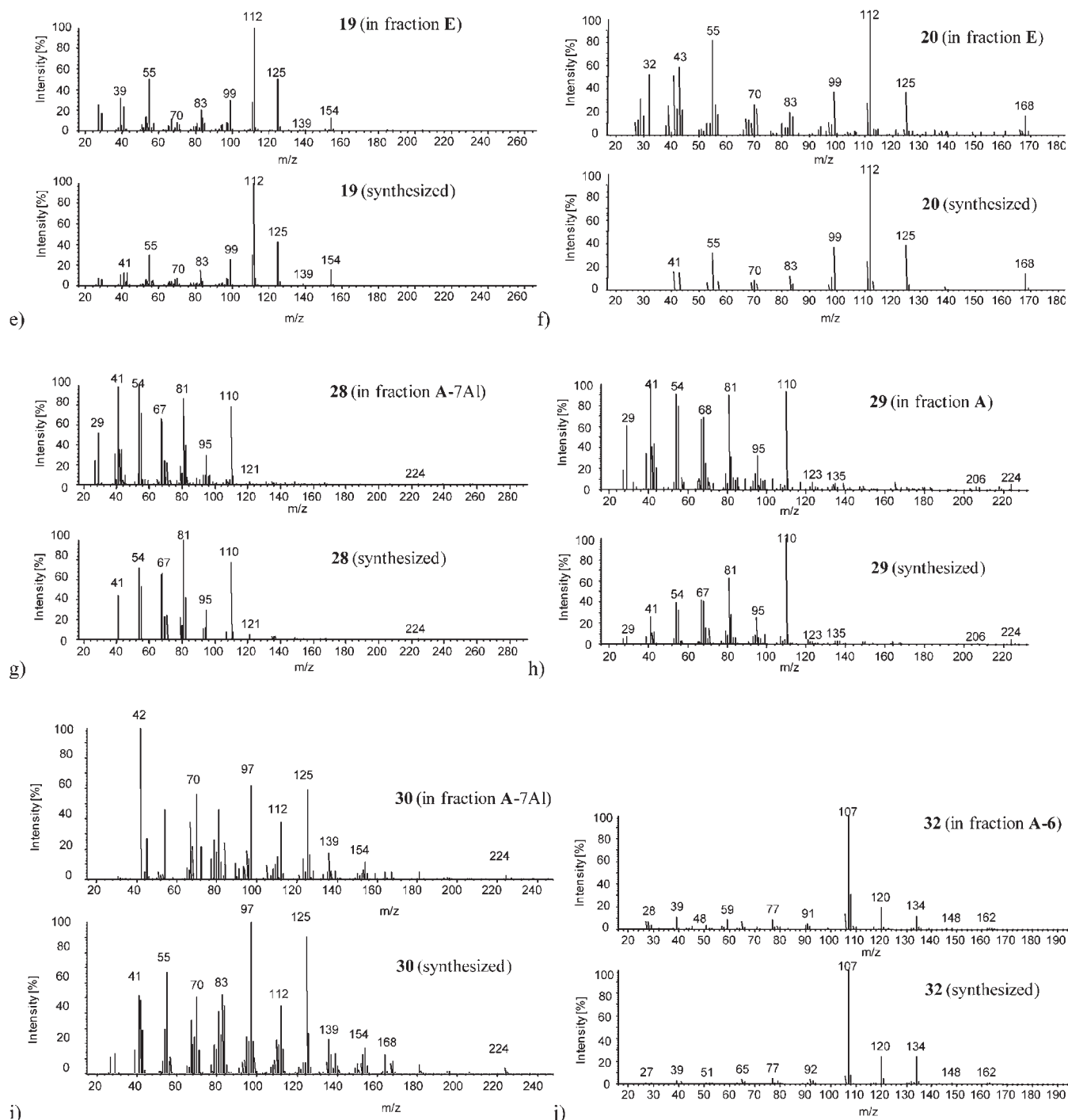
Figure 2. Mass spectra of new molecules identified in chicken and compared with those of the synthetic reference: (a) 5-propyl-1-cyclopentene-1-carbaldehyde 6 ; (b) 5-pentyl-1-cyclopentene-1-carbaldehyde 7 ; (c) high-resolution GC-TOF-MS obtained on 12 in chicken extract E; (d) ( E )-3-(5-ethylcyclopent-1-enyl)acrylaldehyde 12 ; (e) 3-butyl-2-hydroxy-2-cyclopenten-1-one 19 ; (f) 2-hydroxy-3-pentyl-2-cyclopenten-1-one 20 ; (g) (8 Z )-8-tetradecen-5-olide 28 ; (h) (8 E )-8-tetradecen-5-olide 29 ; (i) (6 E )-6-tetradecen-5-olide 30 ; (j) 4-methyl-2-pentylpyridine 32 .
