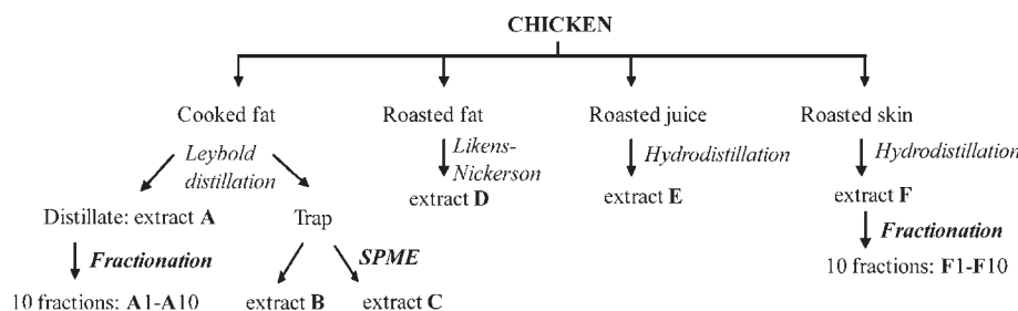
Figure 1. Extraction of the chicken parts (skin, fat, juice) investigated separately for their volatile composition. A = cooked fat Leybold distillate extract; B = cooked fat Leybold trap extract; C = cooked fat Leybold solid-phase microextraction (SPME) extract; D = roasted fat (Likens–Nickerson) extract; E = roasted juice hydrodistillate extract; F = roasted skin hydrodistillate extract.
