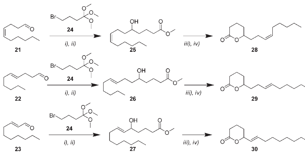
Scheme 4. Synthesis of the New \delta -Lactones ( 8Z )-Tetradecen-5-olide 28, ( 8E )- \epsilon -Tetradecen-5-olide 29, and ( 6E )-Tetradecen-5-olide 30 Identified in Chicken Fat a
