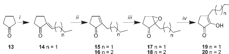
Scheme 3. Synthesis of 3-Butyl-2-hydroxy-2-cyclopenten-1-one 19 and 2-Hydroxy-3-pentyl-2-cyclopenten-1-one 20 a
