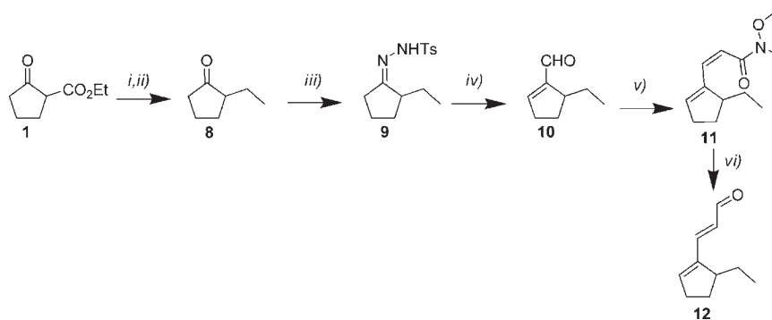
Scheme 2. Synthesis of ( E )-3-(5-Ethyl 1-cyclopentenyl)propenal 12 a
